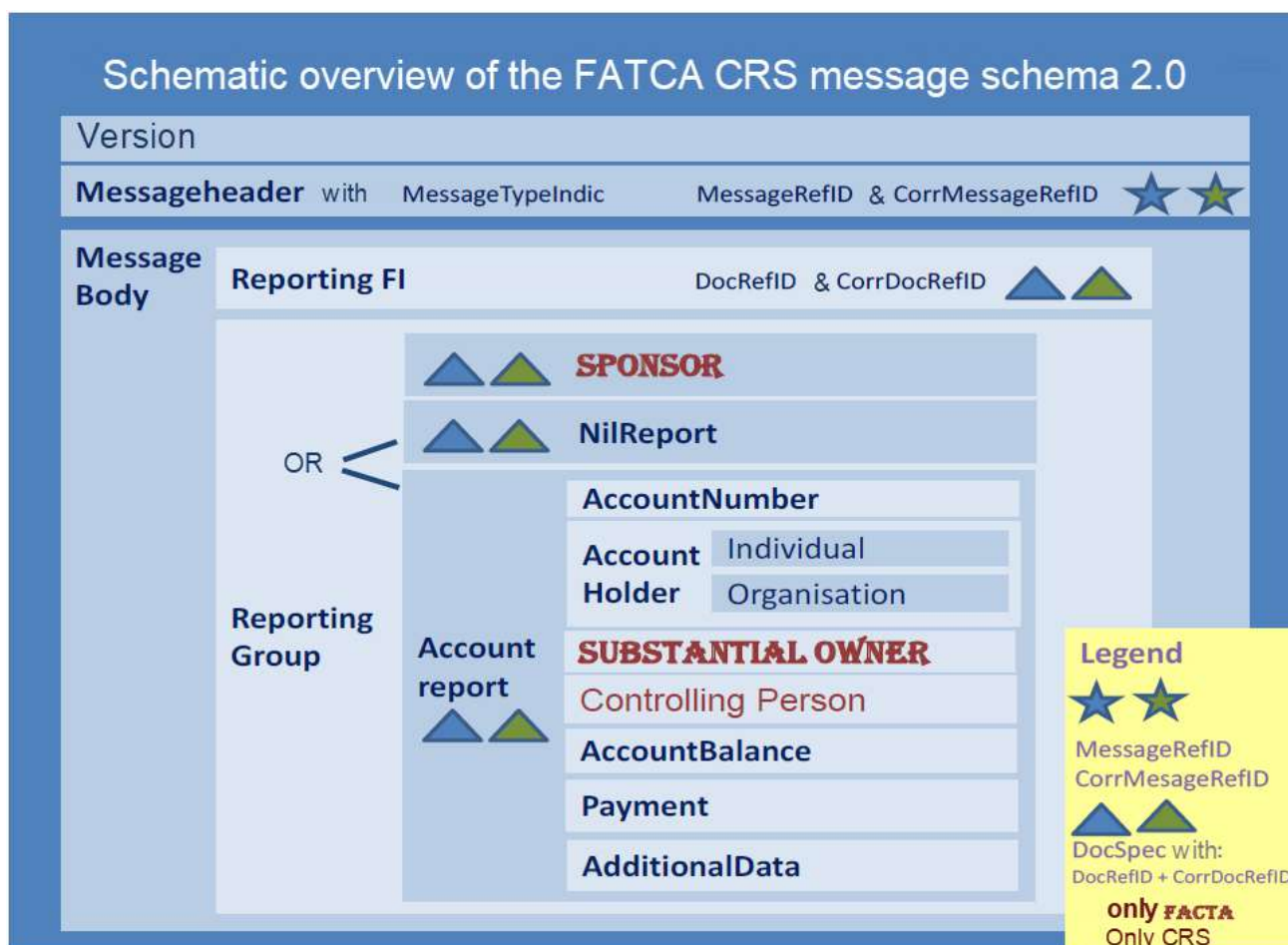
Figure 1a: Schematic overview of the FATCA CRS XML message schema 2.0
