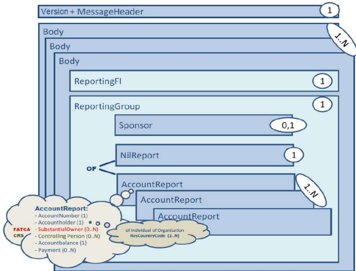
Figure 1b: Cardinality within the FATCA CRS XML message schema 2.0
